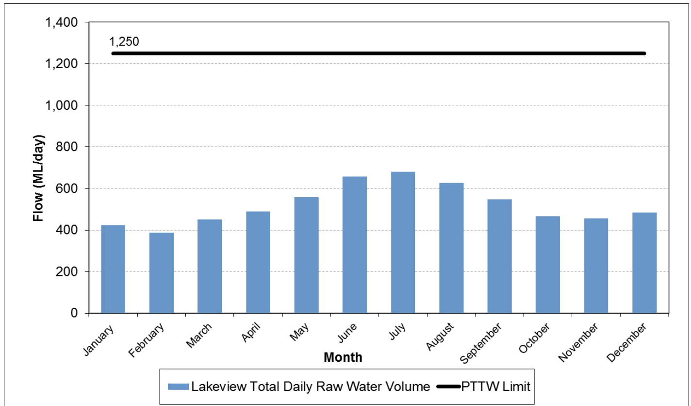
Figure 3: 2018 Lakeview Maximum Daily Raw Water Volumes
