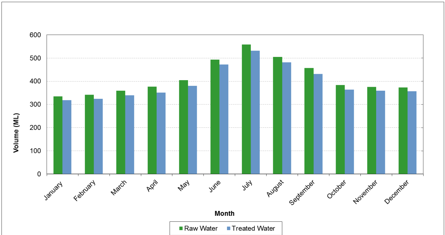
Figure 2: 2018 Lakeview Average Daily Water Production
