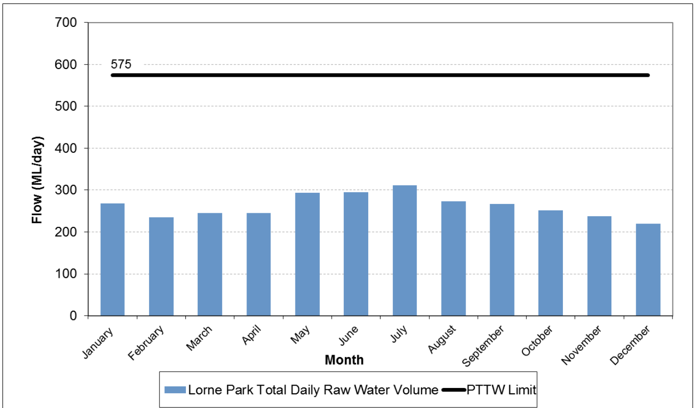
Figure 7: 2018 Lorne Park Maximum Daily Raw Water Volumes
