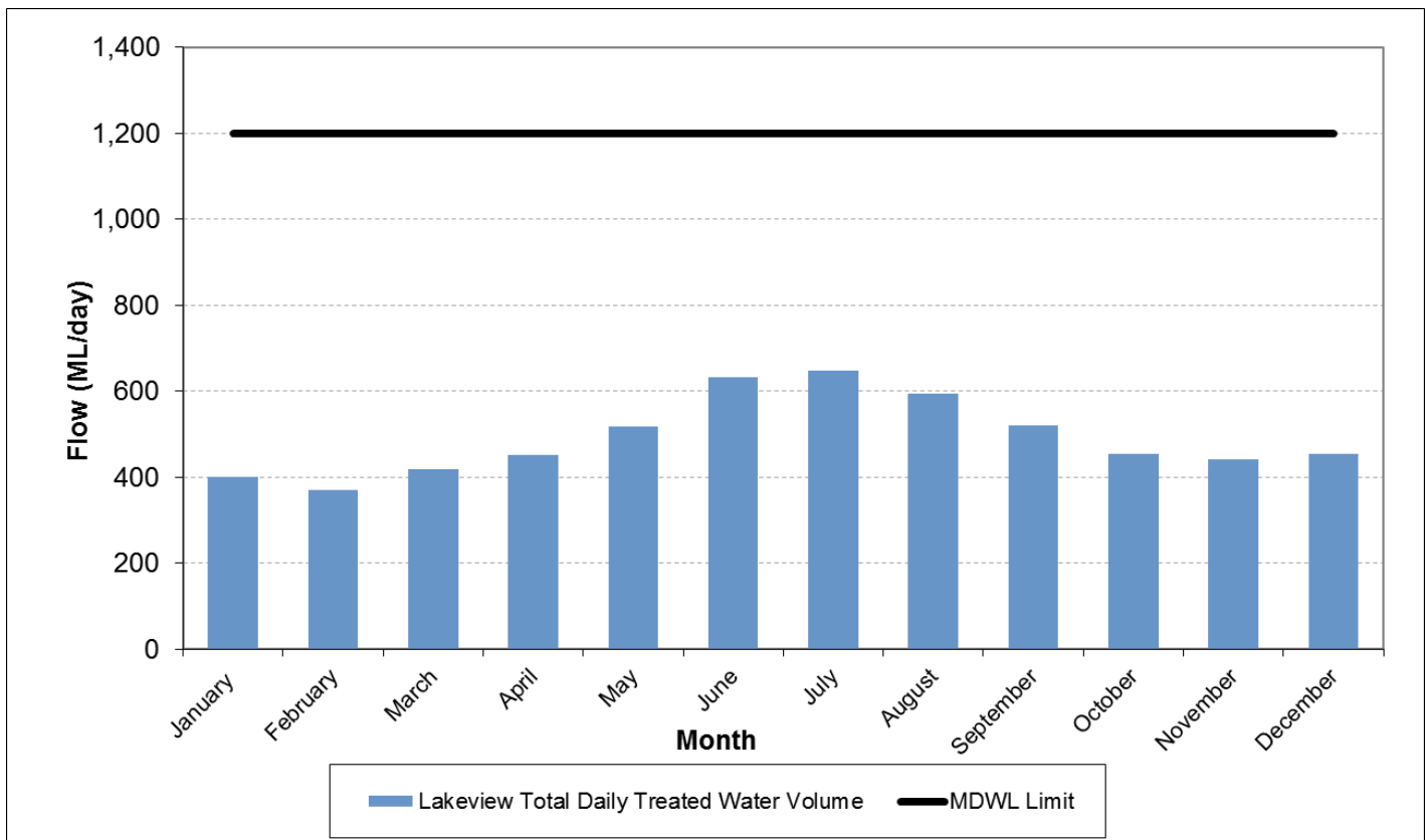
Figure 4: 2018 Lakeview Maximum Daily Treated Water Production
