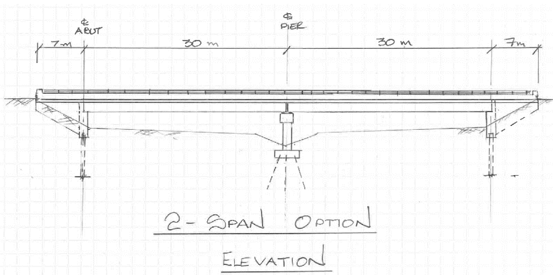
Figure 5-17: Conceptual Cross-Section for Structural Alternative 2C
