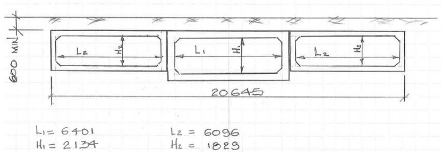
Figure 5-14: Conceptual Cross-Section for Structural Alternative 2A - South Structure
