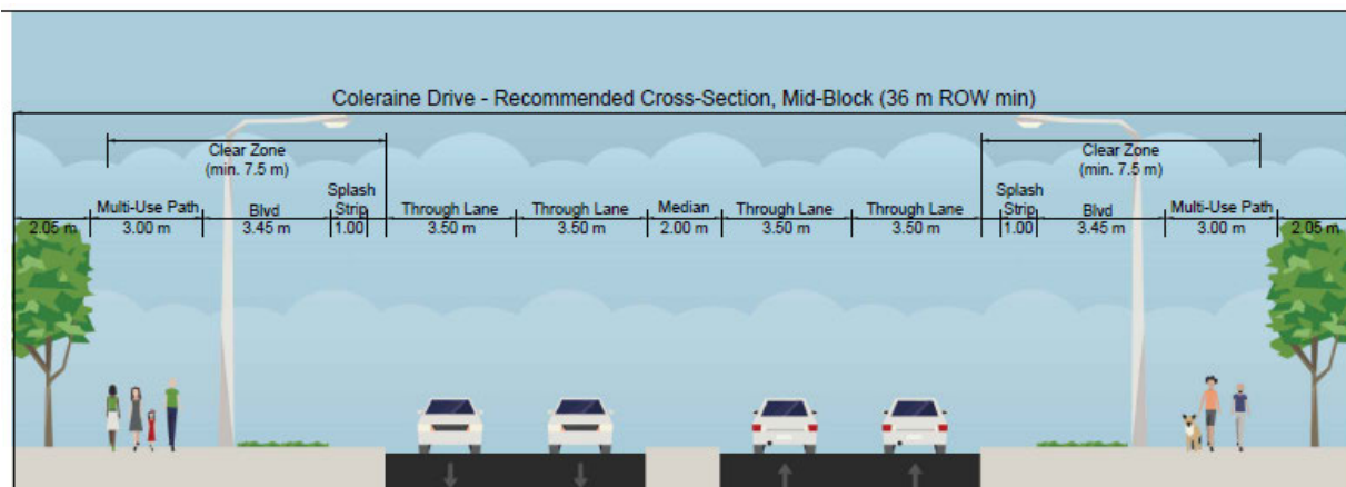
Figure 6-4: Coleraine Drive – Recommended Cross-Section, Mid-Block
