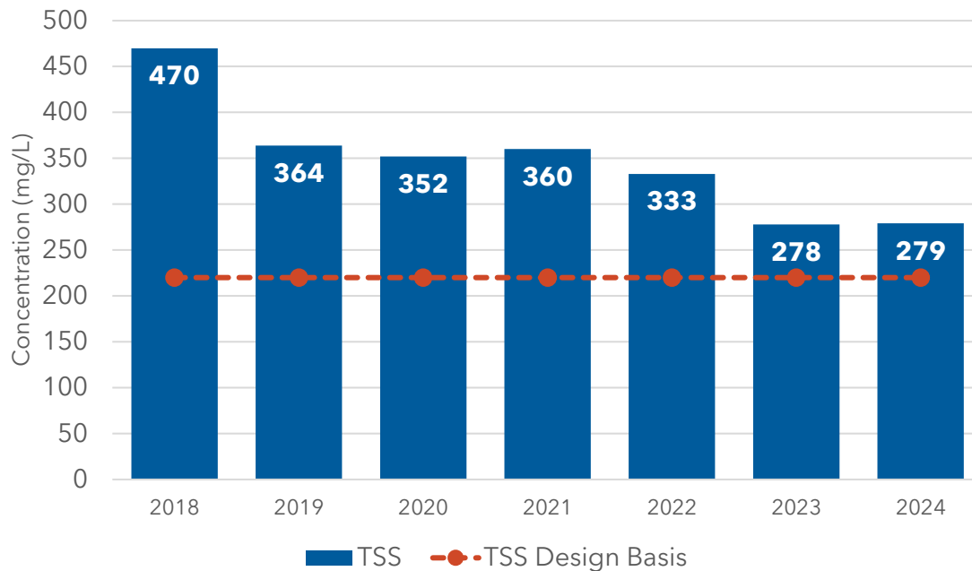
Figure 7. Influent TSS
