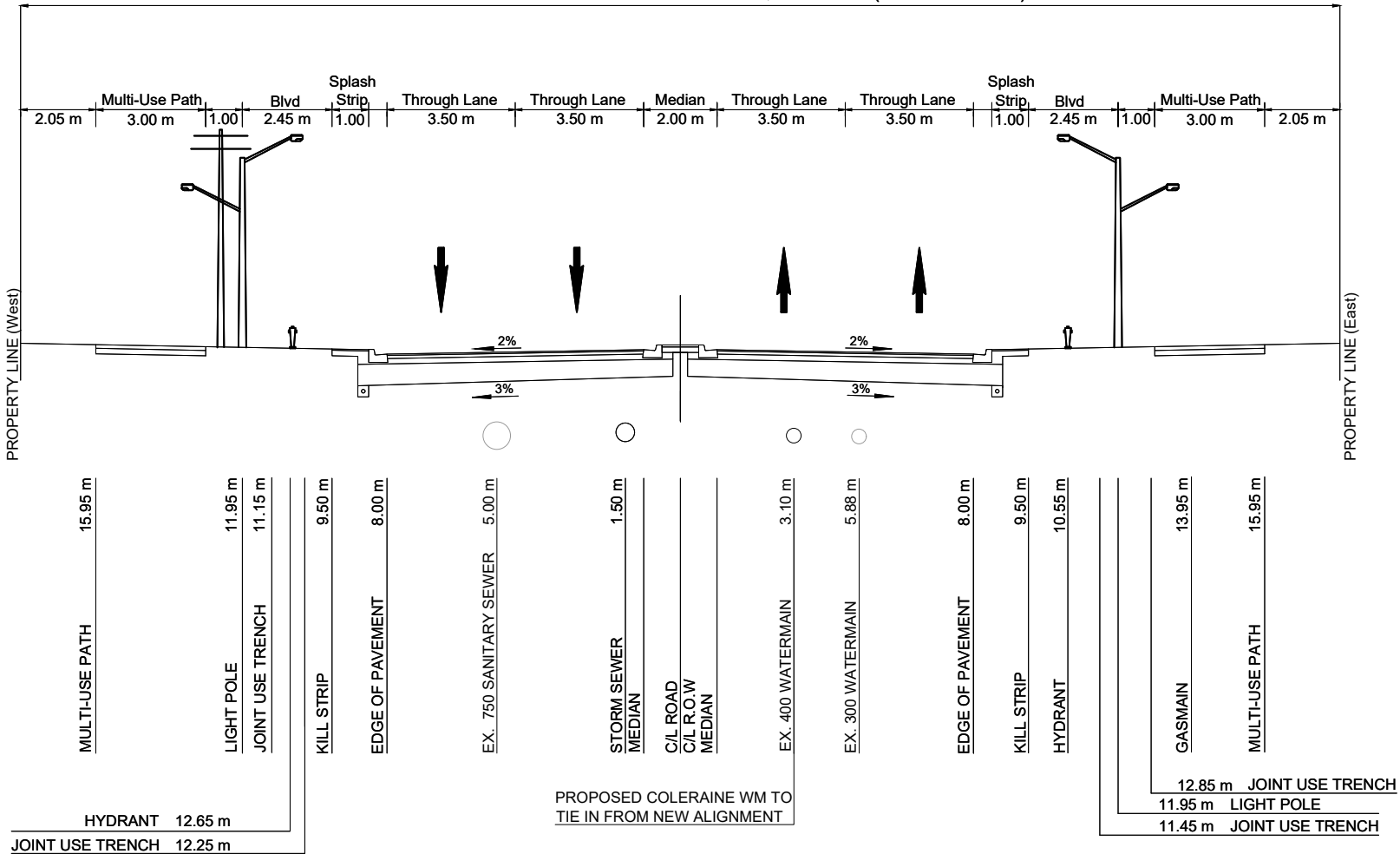
Coleraine Drive - Recommended Cross-Section, Mid-Block (36 m ROW min)
