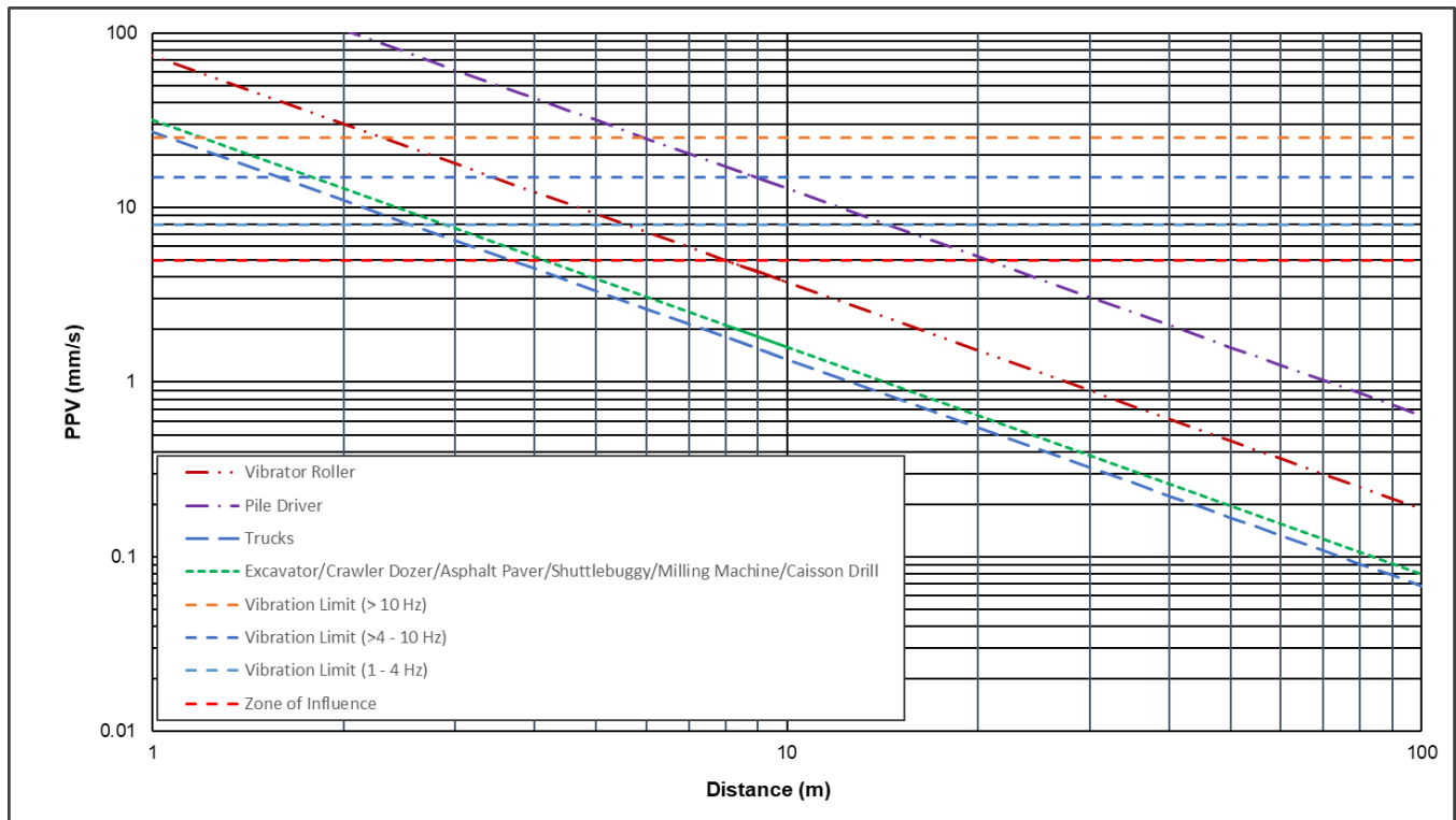
Figure 3: Ground Vibration Attenuation Model for the Proposed Construction Operations
