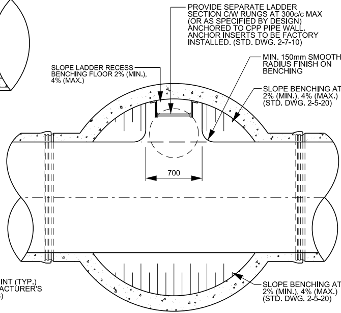
TYPICAL BENCHING PLAN (REDUCED SCALE) AT LADDER RECESS
