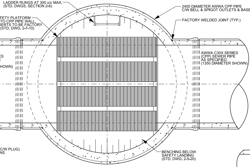
TYPICAL PLAN SECTION (LADDER RECESS NOT SHOWN)
