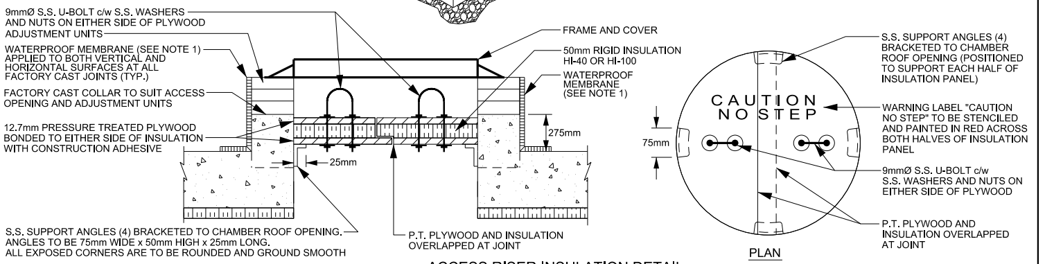
ACCESS RISER INSULATION DETAIL
