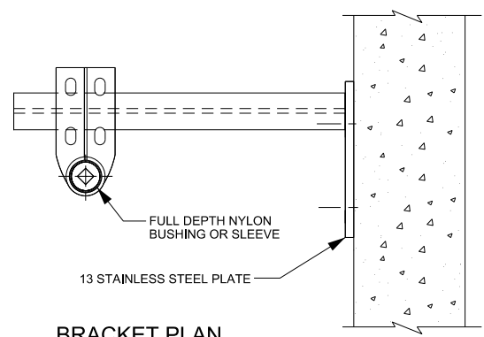
BRACKET PLAN
