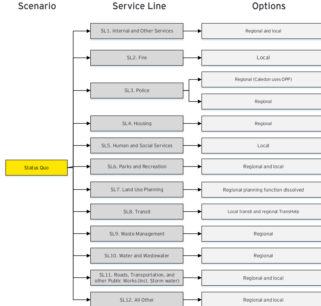
Figure 1. Parameters of the Status Quo Model
