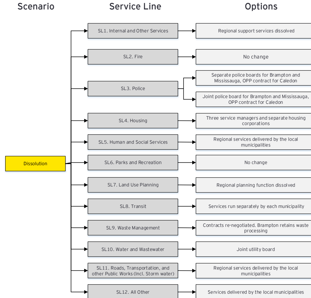
Figure 3. Parameters of the Dissolution Model
